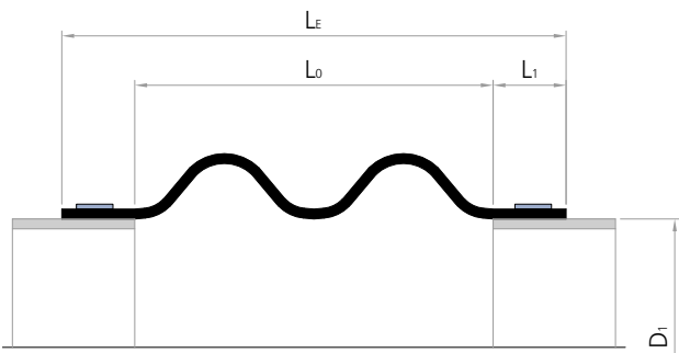
Cross section B120
