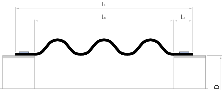
Cross section B130
