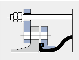
Type D110B Tie rods mounted outside in rubber bushing to accommodate pressure thrust forces
