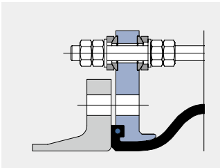
Type D110M Tie rods mounted outside and inside in spherical washers and ball disks to accommodate pressure/vacuum thrust forces
