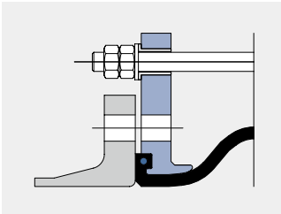
Type D110B Tie rods mounted outside in rubber bushing to accommodate pressure thrust forces
