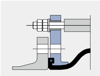
Type D110C Tie rods mounted outside in rubber bushing and inside with compression sleeve to accommodate pressure/vacuum thrust forces
