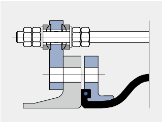
Type D110C Tie rods mounted outside in rubber bushing and inside with compression sleeve to accommodate pressure/vacuum thrust forces
