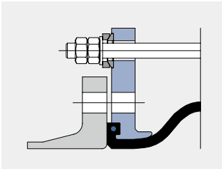
Type D110E Tie rods mounted outside in spherical washers and ball disks to accommodate pressure thrust forces
