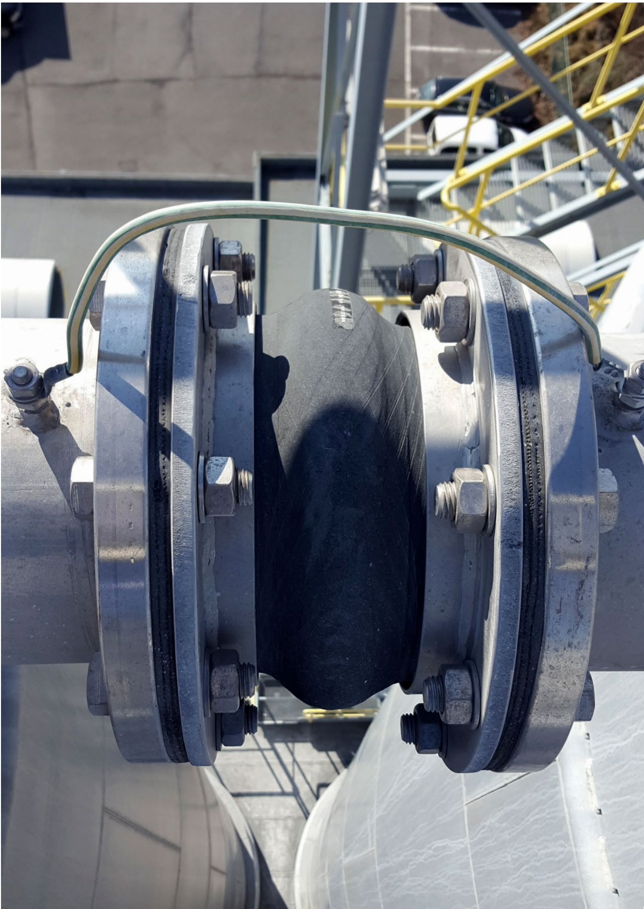
Type U110A single arch rubber expansion joint Ø 300 mm PN6
