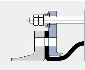
Type U110E Tie rods mounted outside in spherical washers and ball disks to accommodate pressure thrust forces
