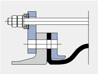
Type U110K Gusset plates: Tie rods mounted outside in spherical washers and ball disks to accommodate pressure thrust forces
