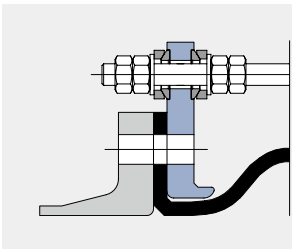
Type U110M Tie rods mounted outside and inside in spherical washers and ball disks to accommodate pressure/vacuum thrust forces
