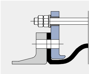
Type U110B Tie rods mounted outside in rubber bushing to accommodate pressure thrust forces
