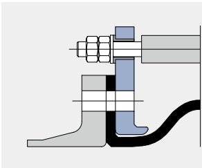
Type U110C Tie rods mounted outside in rubber bushing and inside with compression sleeve to accommodate pressure/vacuum thrust forces
