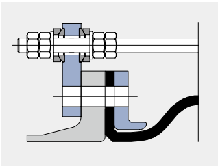
Type U110L Gusset plates: Tie rods mounted outside and inside in spherical washers and ball disks to accommodate pressure/vacuum thrust forces
