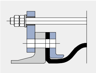
Type U110R Gusset plates: Tie rods mounted outside in rubber bushing to accommodate pressure thrust forces
