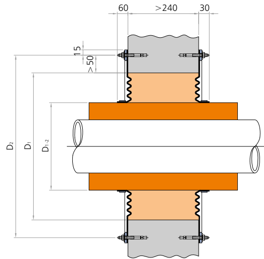
Cross section W200FS + W200FS
