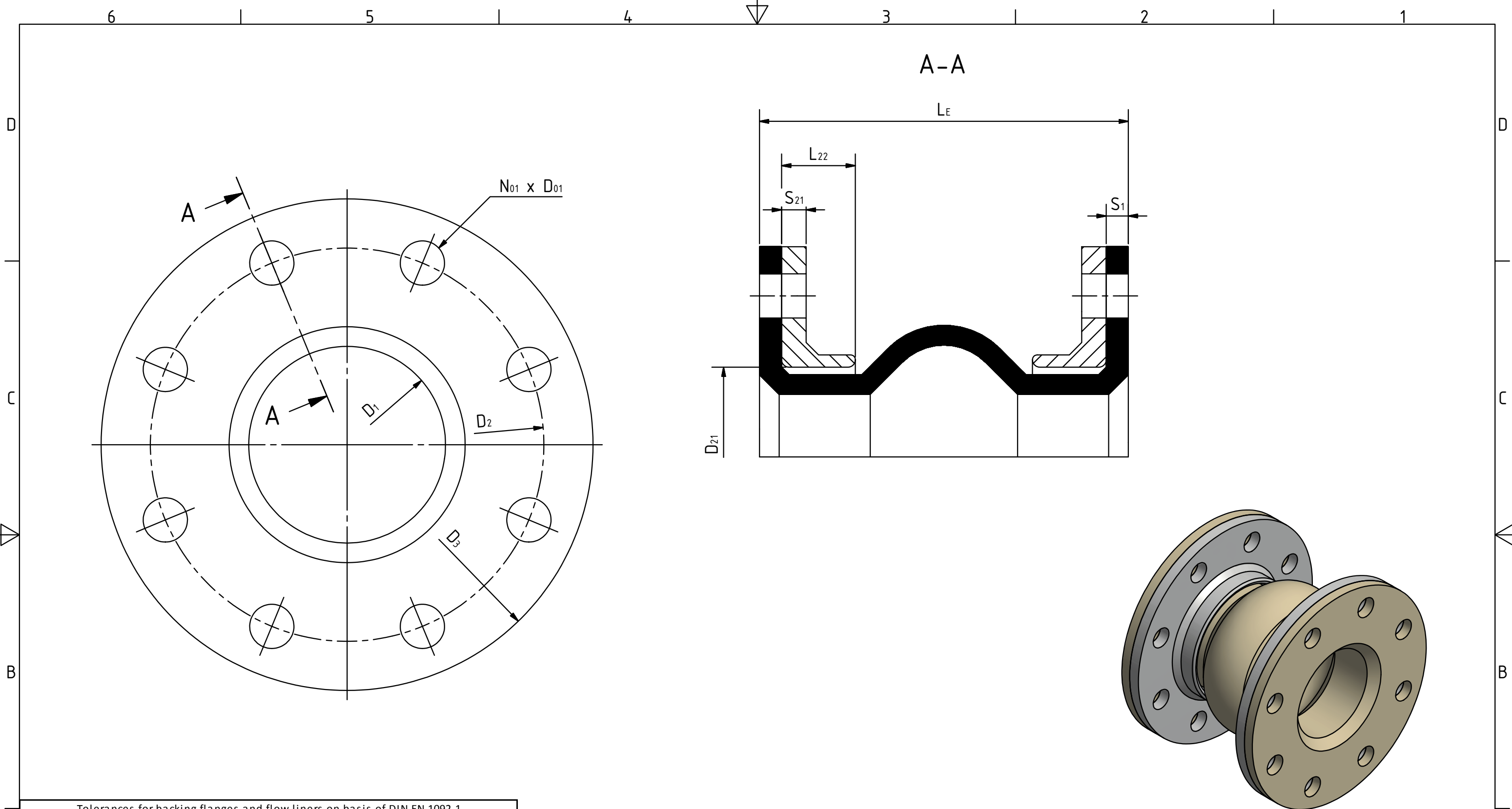
Tolerances for backing flanges and flow liners on basis of DIN EN 1092-1
